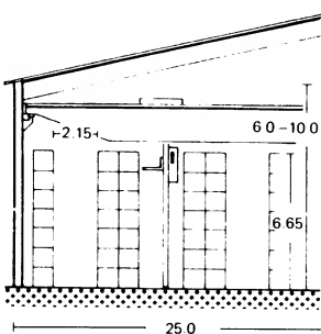
13 With stacker crane
